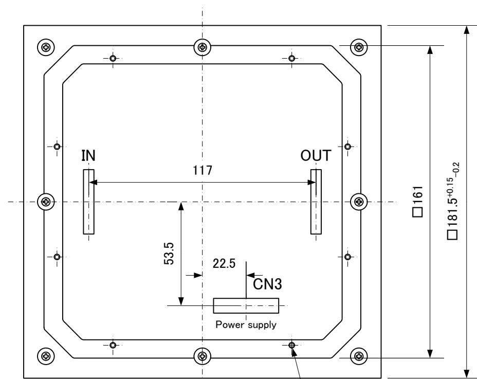
背面/Rear view
